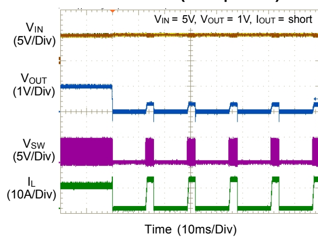
UVP Short (Hiccup Mode)
