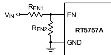
Figure 3. Resistive Divider for Under-Voltage Lockout Threshold Setting
