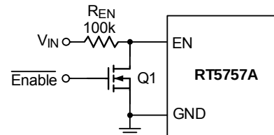
Figure 2. Logic Control for the EN Pin
