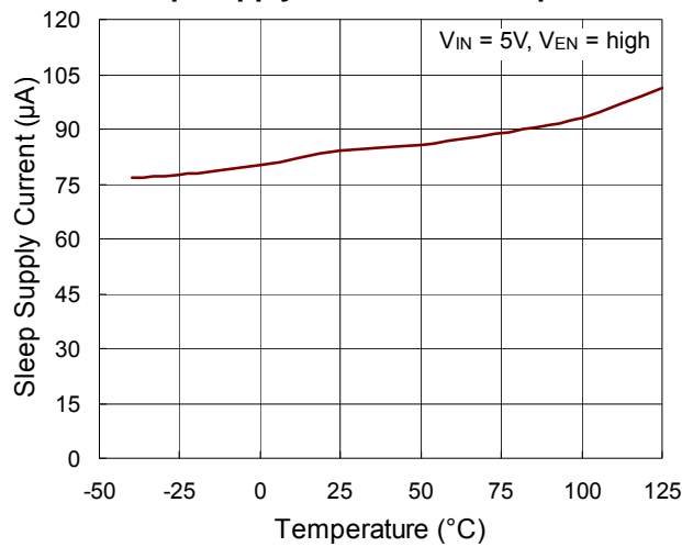
Sleep Supply Current vs. Temperature
