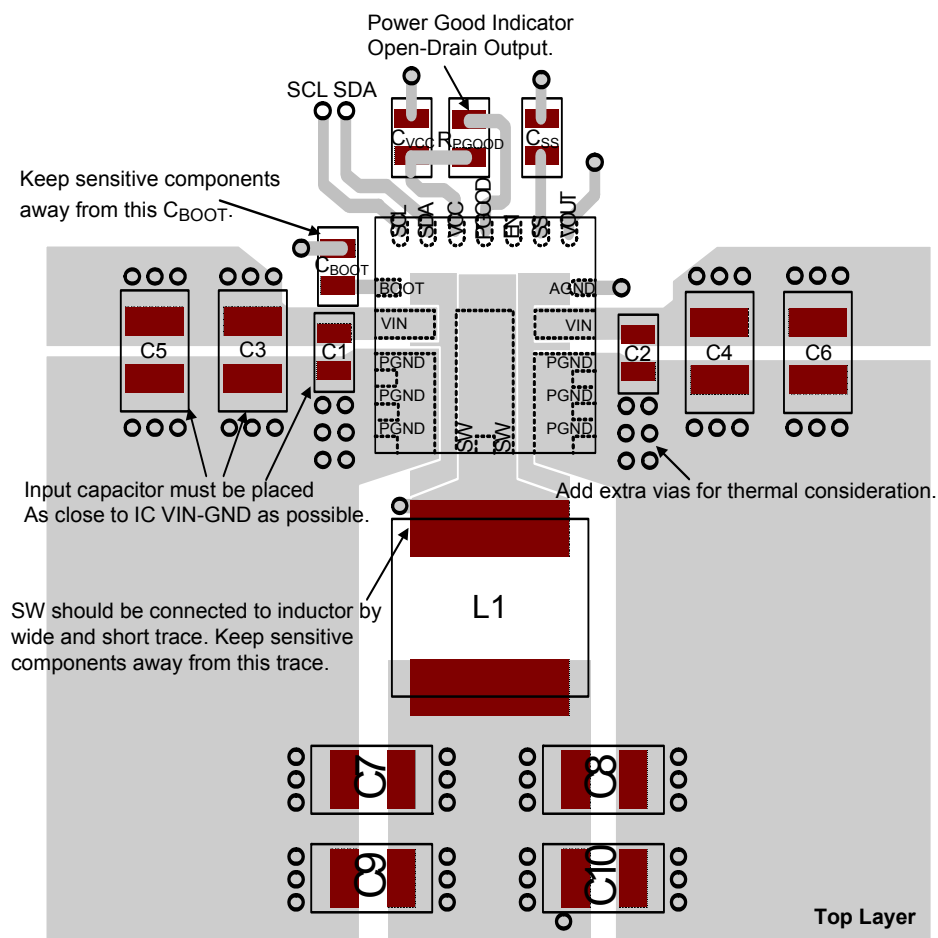
Figure 10. Layout Guide (Top Layer)
