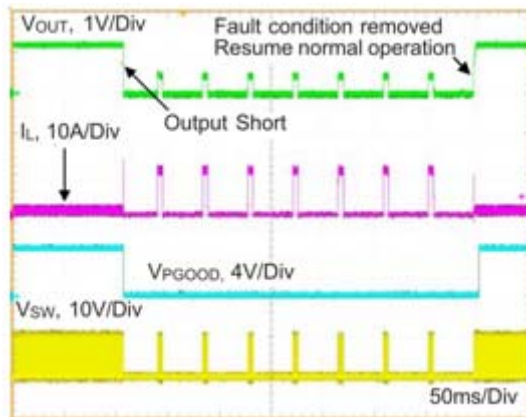
Figure 2. Current Limit and UVP
