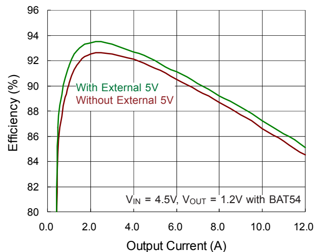
Figure 6. Efficiency Comparison with/without External 5V Supply.
