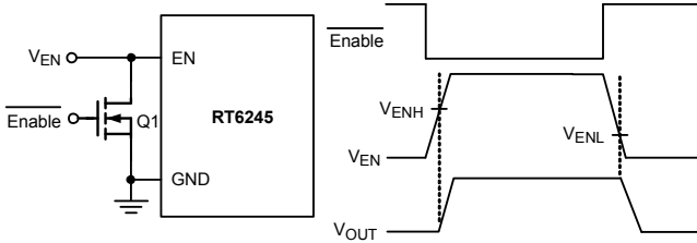
Figure 8. Logic Control for the EN Pin
