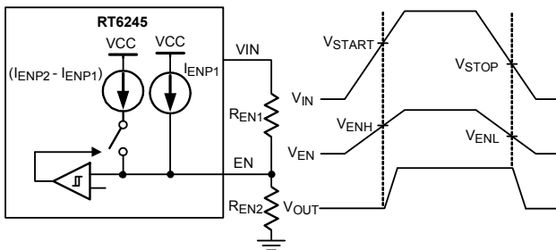
Figure 9. Adjustable VIN UVLO
