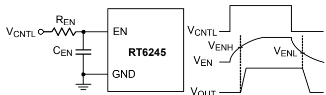
Figure 7. Enable Timing Control
