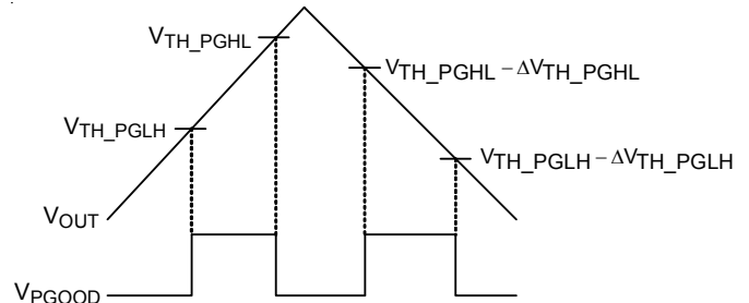
Figure 3. The Logic of PGOOD
