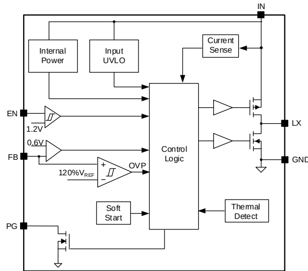
Figure 3. Block Diagram
