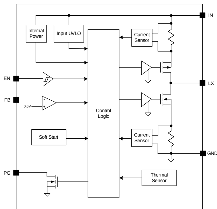
Figure3. Block Diagram
