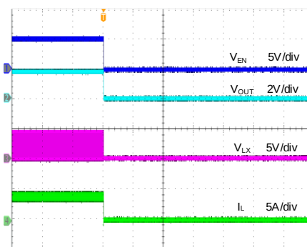
Shutdown from EN ( V_N=5V , V_{OUT}=1.8V , I_{OUT}=4A )
