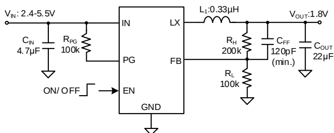
Figure1. Schematic Diagram
