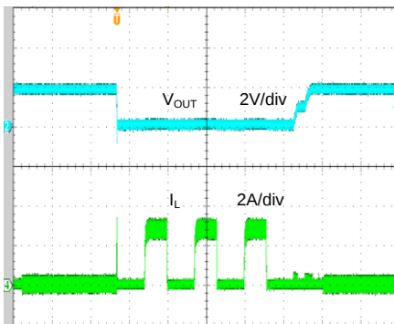
Short Circuit Protection ( V_{IN}=5.0V , V_{OUT}=1.8V , I_{OUT}=0 ~Short)
