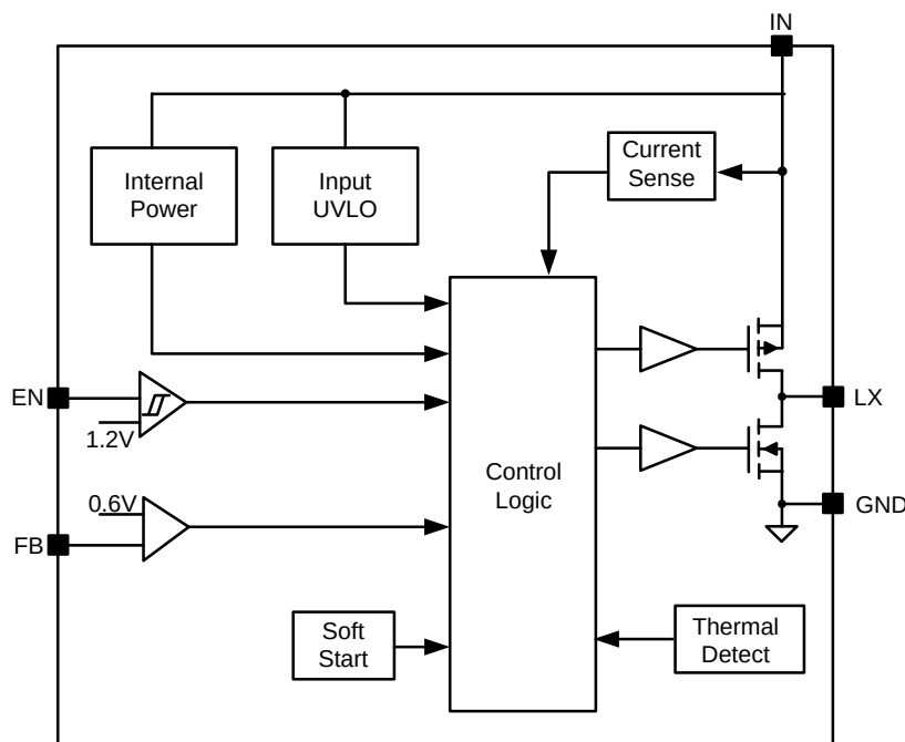
Figure3. Block Diagram
