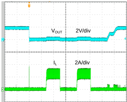
Short Circuit Protection ( V_{IN}=5.0V , V_{OUT}=1.8V , I_{OUT}=0\sim\text{Short} )
