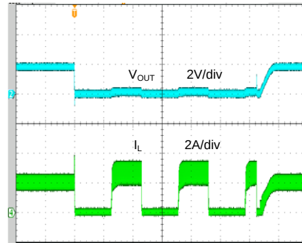
Short Circuit Protection ( V_{IN}=5.0V , V_{OUT}=1.8V , I_{OUT}=2A\sim\text{Short} )
