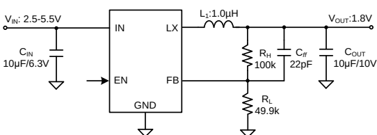
Figure1. Schematic Diagram
