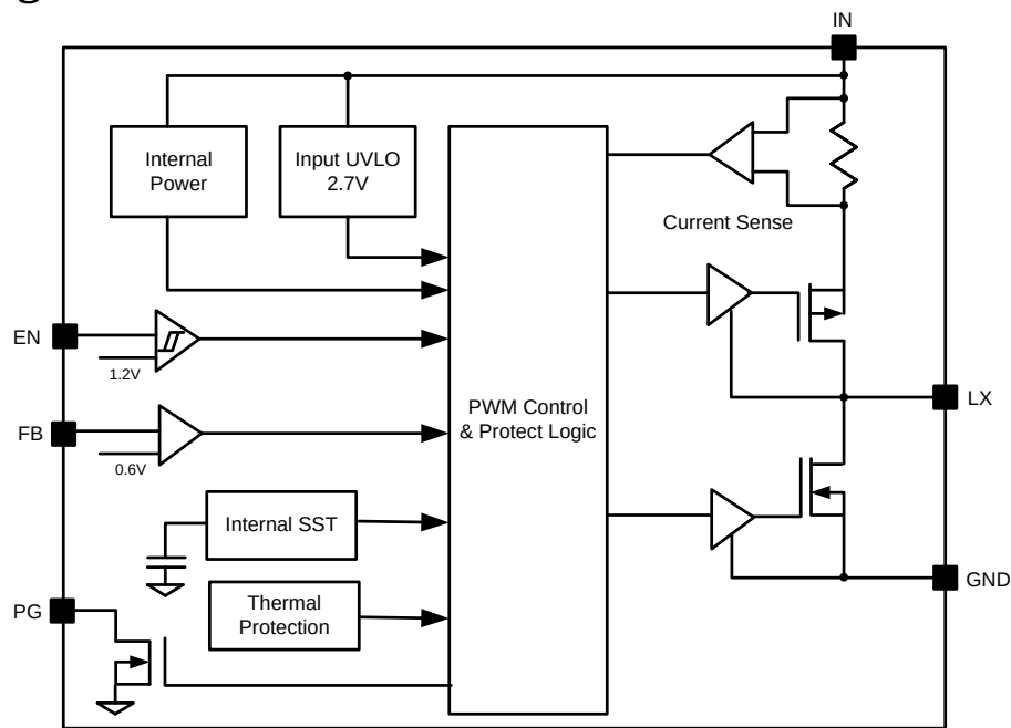
Figure3. Block Diagram
