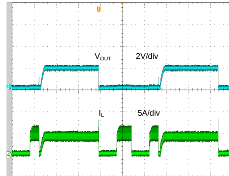
Short Circuit Protection ( V_{IN}=5V , V_{OUT}=1.8V , 4A to Short)
