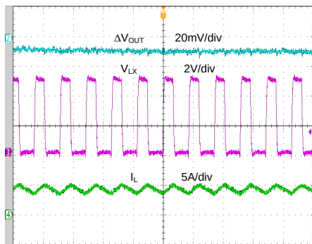
Output Ripple ( V_{IN}=5V , V_{OUT}=1.8V , I_{OUT}=4A )
