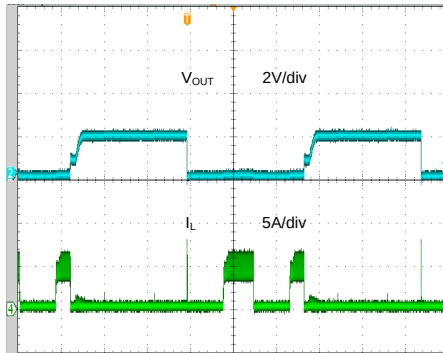
Short Circuit Protection ( V_{IN}=5V , V_{OUT}=1.8V , 0A to Short)
