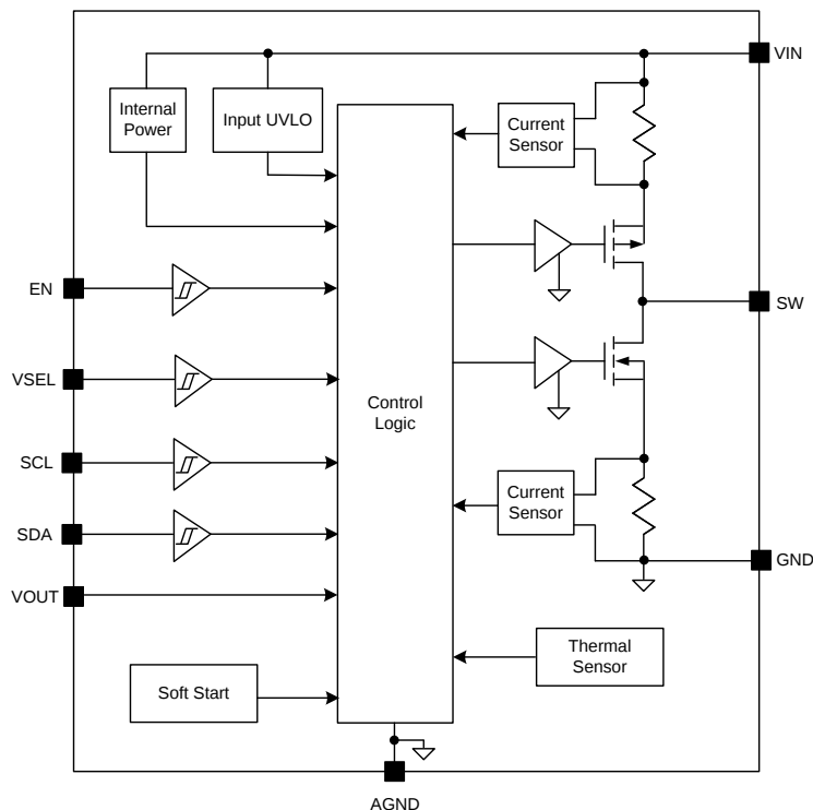
Figure3. Block Diagram
