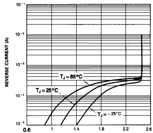
Figure 4. Reverse Characteristics
