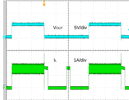
Short Circuit Protection ( V_{IN}=3.3V, V_{OUT}=5V, I_O=1A to Short)
