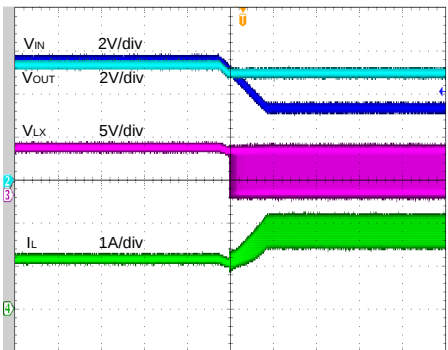
Seamless Transition: Bypass Mode→Boost Mode ( V_{IN}=5.5V\sim3.3V, V_{OUT}=5.0V, I_O=1.0A )
