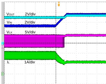
Seamless Transition: Boost Mode→Bypass Mode ( V_{IN}=3.3V\sim5.5V, V_{OUT}=5.0V, I_O=1.0A )
