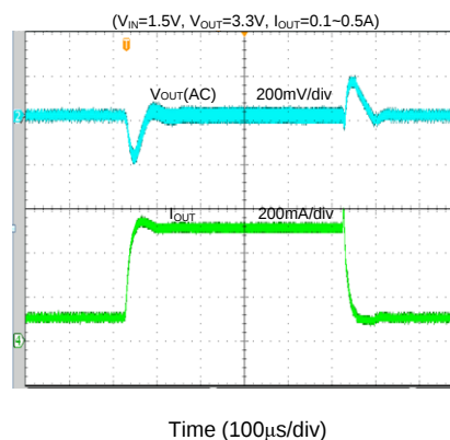
Load Transient
