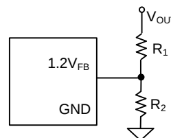
Figure 4. Feedback Resistor Divider
