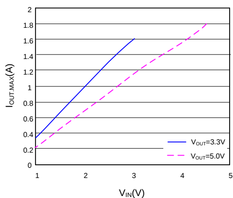
Max load Current VS. V_{IN}
