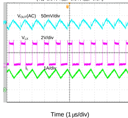
Output Ripple
