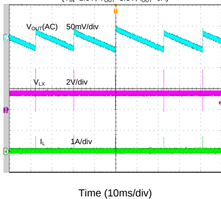
Output Ripple
