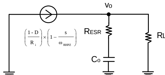
Figure 8. Current Feedback Loop
