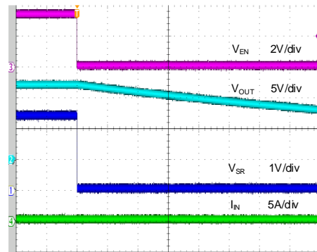
Time (1s/div)
