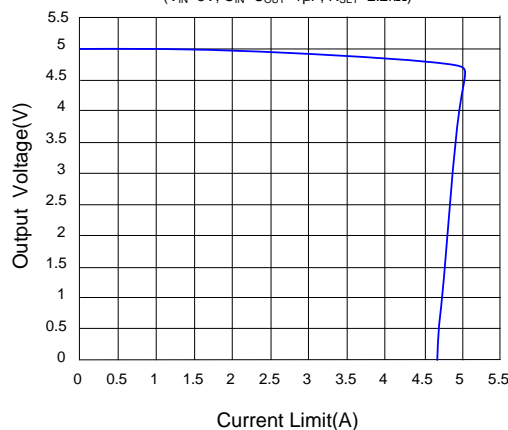
Output Voltage Vs. Current Limit ( V_{IN}=5V , C_{IN}=C_{OUT}=1\mu F , R_{SET}=2.2k\Omega )
