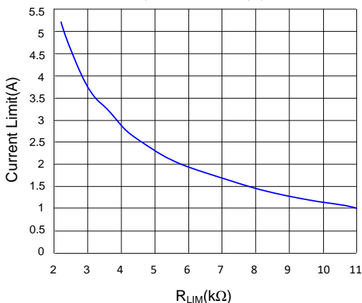
Current Limit vs. R_{LIM} ( V_{IN}=5V , C_{IN}=C_{OUT}=1\mu F )
