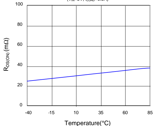
R_{DS(ON)} vs. Temperature ( V_{IN}=5V , I_{LOAD}=0.5A )
