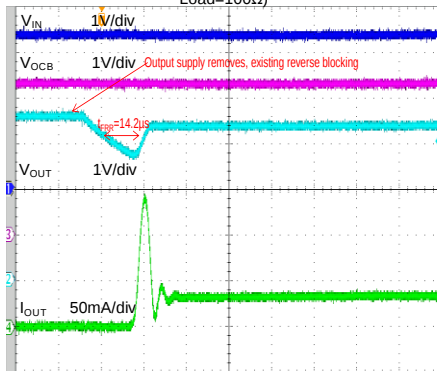
Fast Reverse Blocking Recovery Response (V_{IN}=3.3V, V_{OUT}=3.5V \text{ removes}, C_{IN}=1nF, C_{OUT}=1\mu F, \text{Load}=100\Omega)
