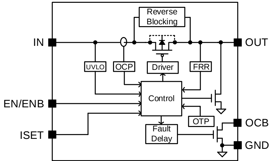
Figure2. Block Diagram
