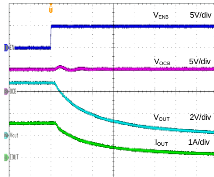
Shutdown from Enable ( V_{IN}=5V , C_{IN}=C_{OUT}=10\mu F , 1.5A Load, SQ24201E2)
