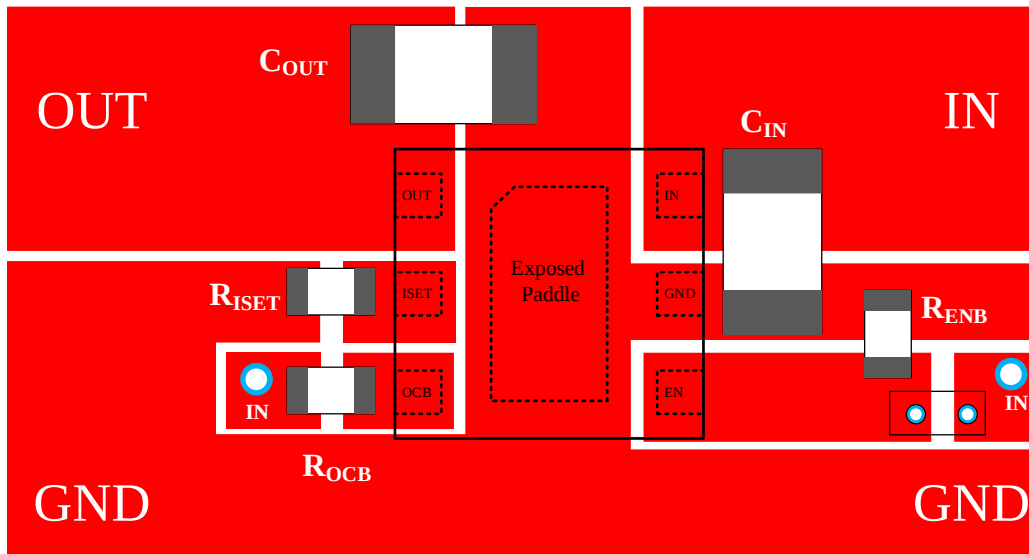
Figure3 (a). PCB Layout Suggestion (SQ24201EDED/SQ24201E2DED)
