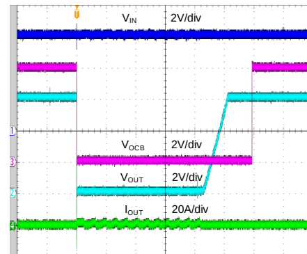
Short Circuit (V_{IN}=6V, R_{ISET}=15k\Omega (1.7A))
