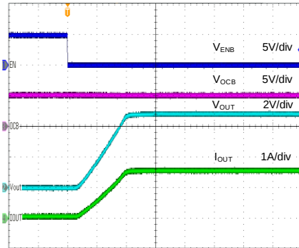
Startup from Enable ( V_{IN}=5V , C_{IN}=C_{OUT}=10\mu F , 1.5A Load, SQ24201E2)
