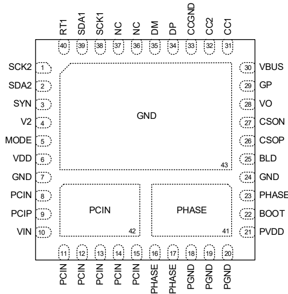
WQFN-42L 6x6
