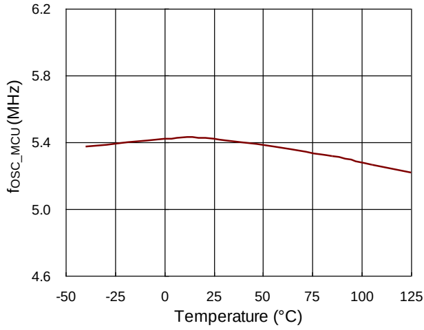
f OSC_MCU vs. Temperature
