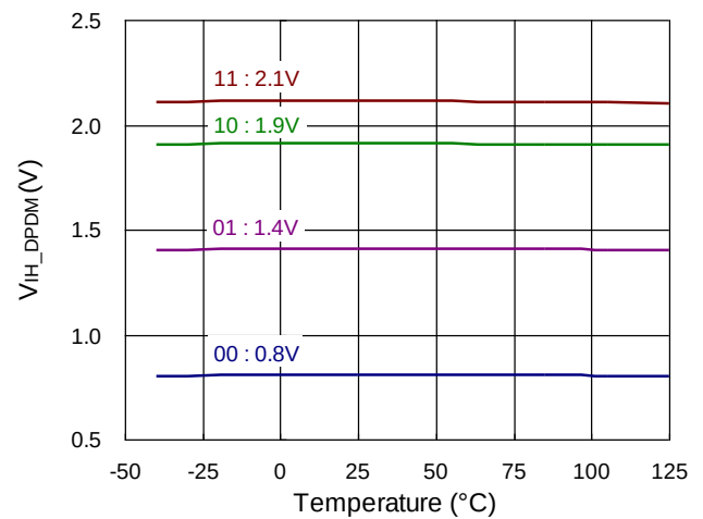
V IH_DPDM vs. Temperature
