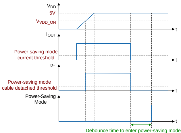
Figure 5. The Bias Voltages Sequence during Start-Up
