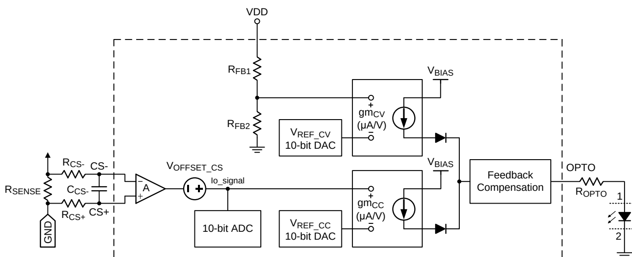
Figure 4. CV and CC Loops
