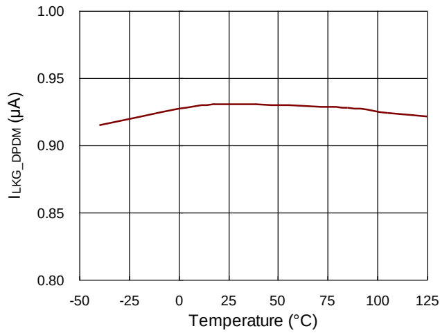
I LKG_DPDM vs. Temperature
