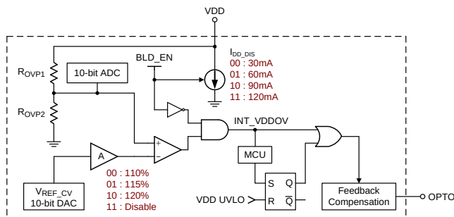
Figure 9. OVP Functional Diagram
