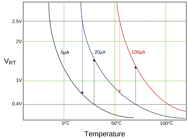
Figure 10. The RT Voltages vs. Temperature at Three Bias Currents
