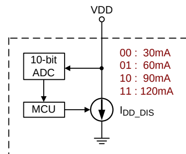
Figure 7. Discharge Current Control from VDD Pin
