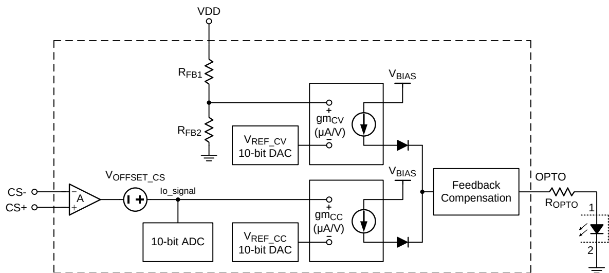
Figure 1. CV/CC Loops and Current Sense
