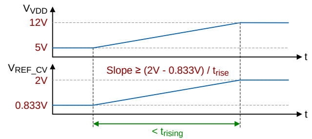
(a) Output Voltage Rising
