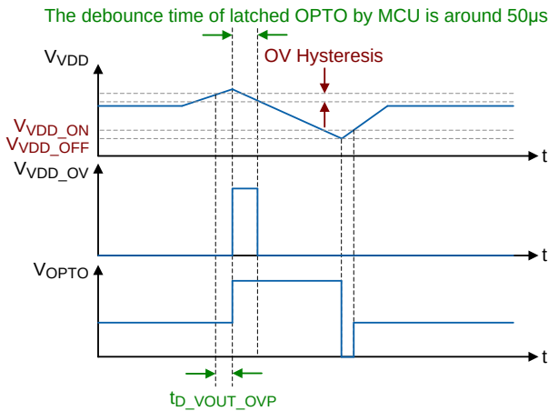
Figure 8. Timing Sequence of the OVP Function
