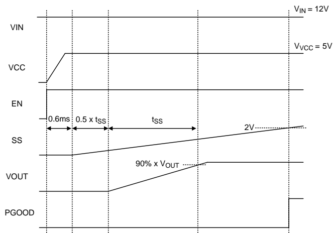
Figure 2. Start-Up Sequence
