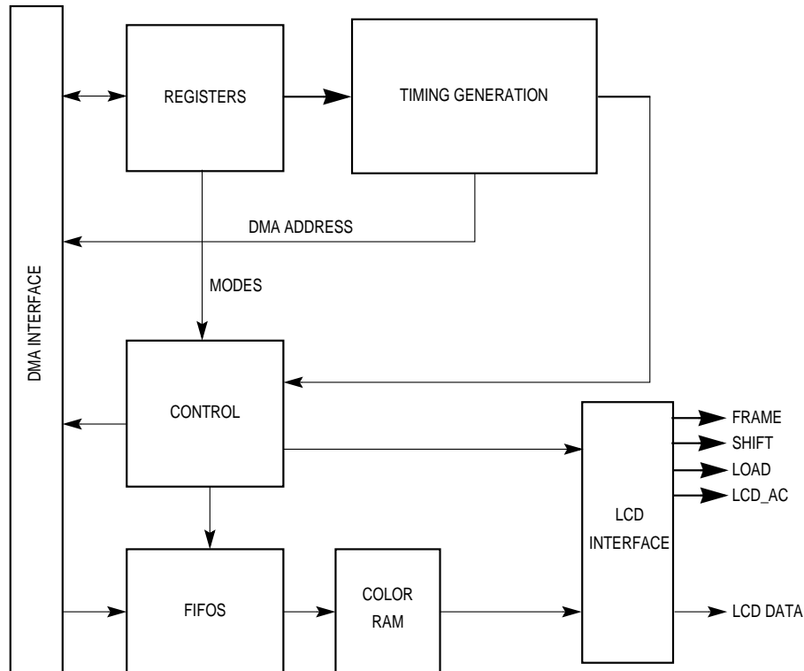
Figure 18-6. LCD Controller Block Diagram
