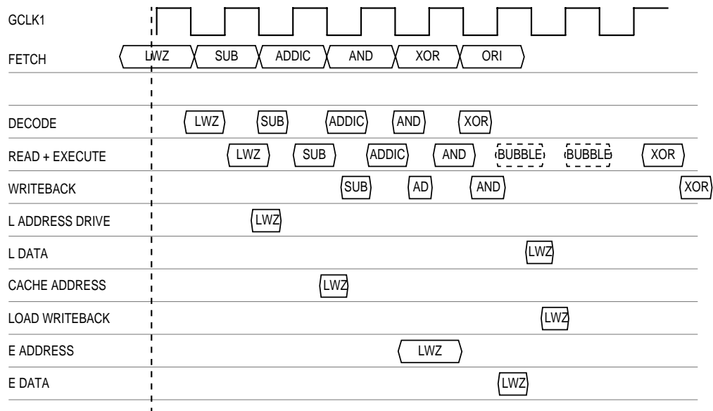
Figure 8-6. Example of a Full History Buffer
