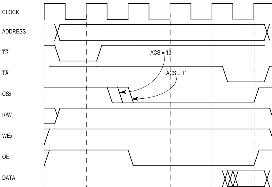
Figure 15-9. MPC823e GPCM-Relaxed Timing-Read Access (ACS = 10 or 11, SCY = 1, and TRLX = 1)
