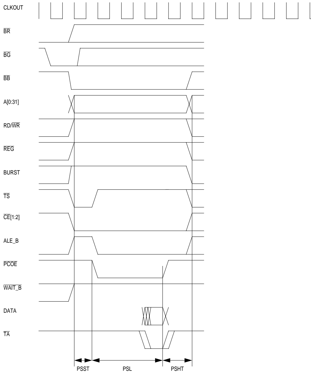
Figure 17-3. PCMCIA Single Beat Read Cycle (PR = 0, PSST = 1, PSL = 3, PSHT = 1)
