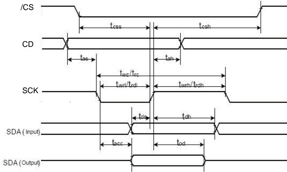
Display Serial Interface Timing Characteristics (4-line SPI system)
