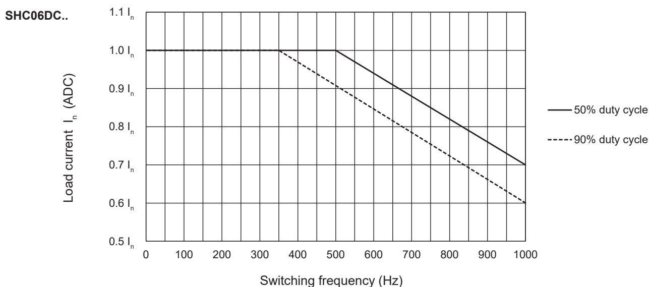
Fig. 4 Current Derating vs. Switching Frequency
