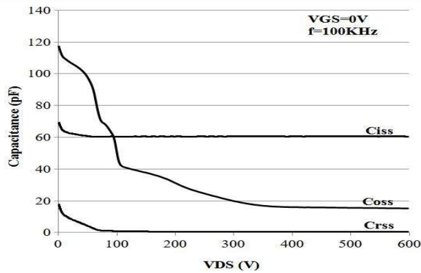
Capacitance vs. V_{DS} Curve @ T_J = 25^{\circ}\text{C}
