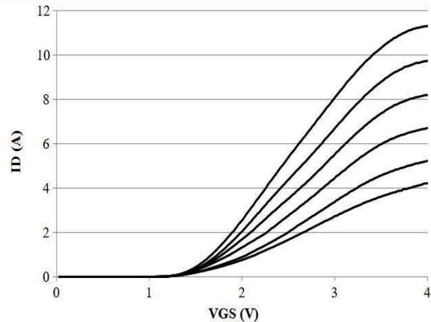
I_{DS} vs. V_{GS} @ T_j = 25^\circ\text{C} - 150^\circ\text{C} , step 25^\circ\text{C}
