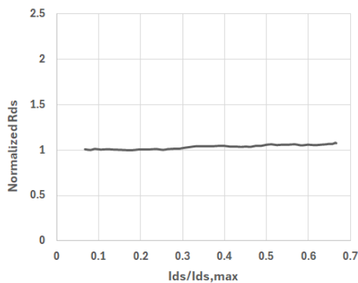
Normalized R_{DS(on)} vs. I_{DS} @ T_J = 25^{\circ}\text{C}
