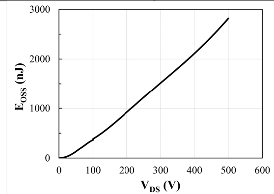
Stored Energy Characteristic E_{OSS} vs. V_{DS}
