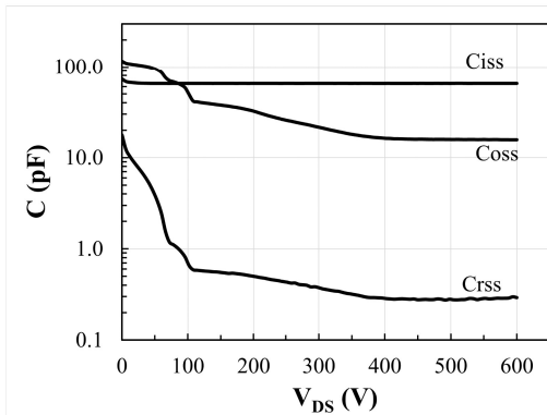
Capacitance vs. V_{ds} Curve @ T_j = 25\text{ }^{\circ}\text{C}
