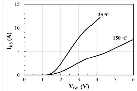
I_{DS} vs. V_{GS} @ T_j = 25\text{ }^{\circ}\text{C} and 150\text{ }^{\circ}\text{C}
