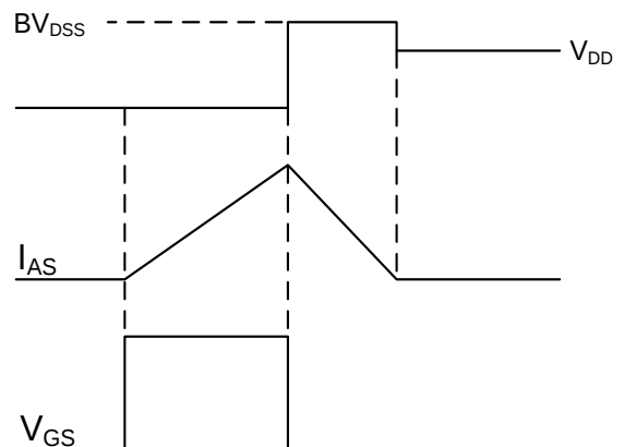
Fig.11 EAS Waveform
