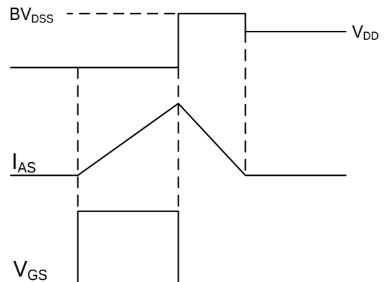
Fig.11 EAS Waveform
