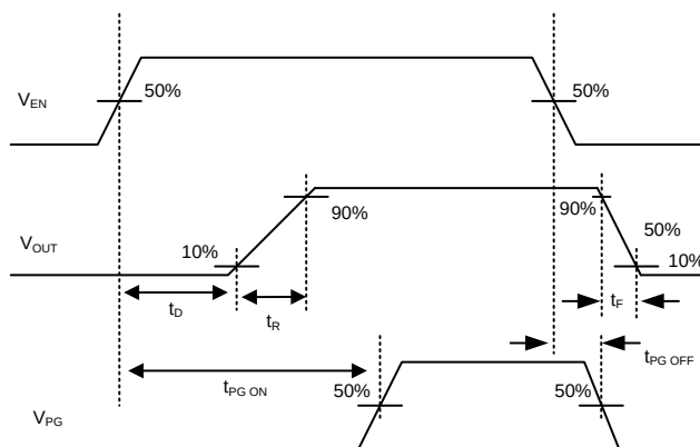
Figure 3. Timing Waveform
