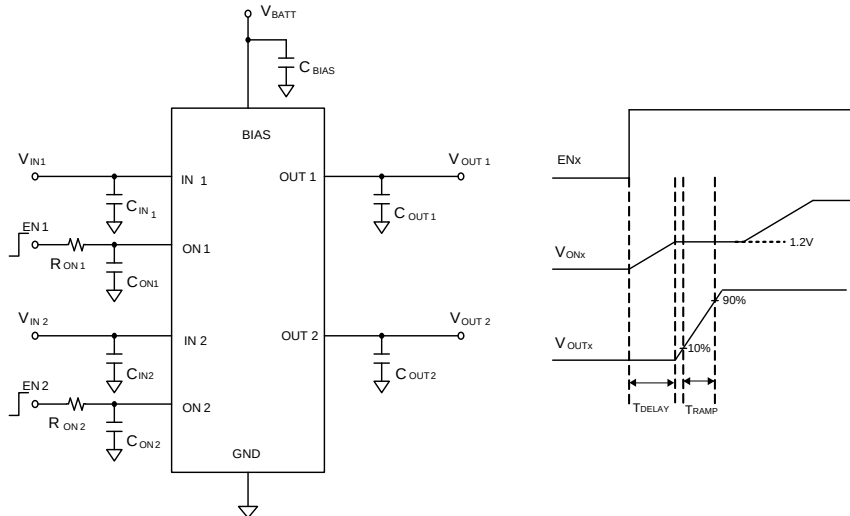
Figure 1. Schematic Diagram
