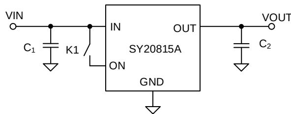
Figure 4. Schematic Diagram
