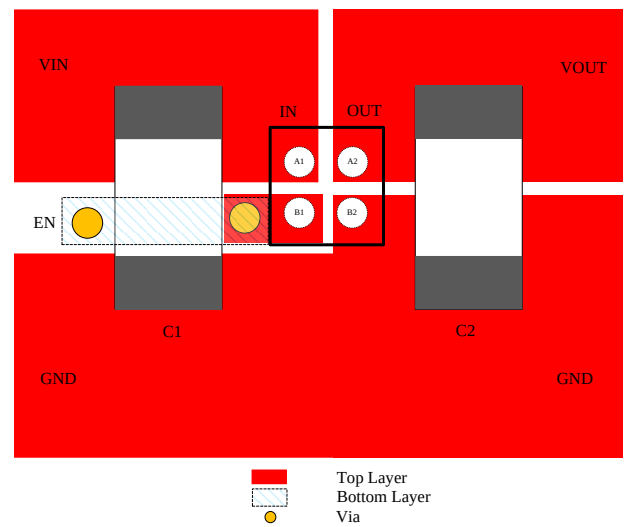
Figure 3. PCB Layout Suggestion
