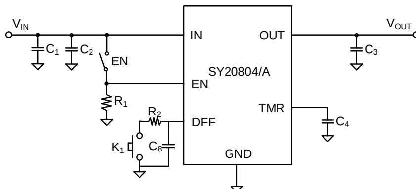
Figure 6. Application Schematic
