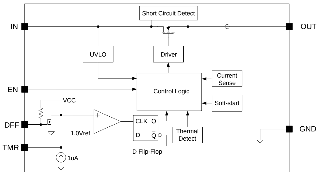
Figure 2. Block Diagram
