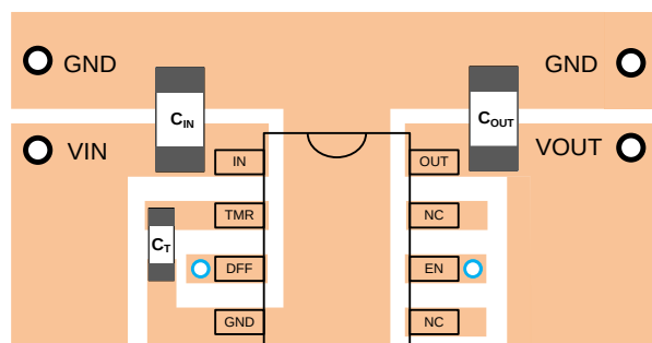
Figure 5. PCB Layout Suggestion
