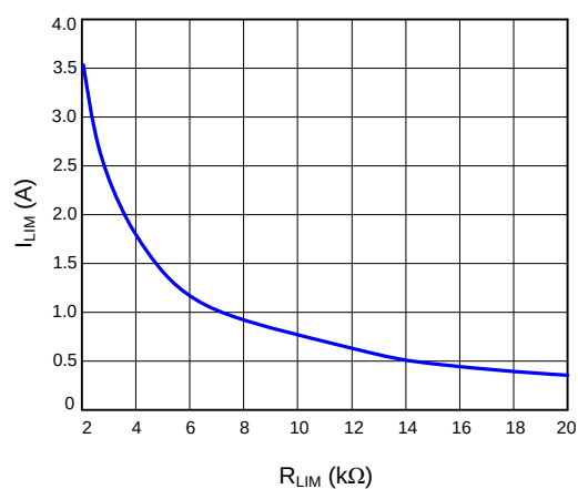
R_{LIM} vs. I_{LIM}
