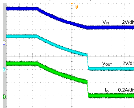
Shutdown from V_{IN} ( V_{IN}=3.3V , I_O=0.5A )
