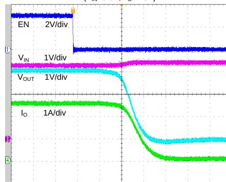
Shutdown from Enable ( V_{IN}=3.3V , I_O=2.5A )
