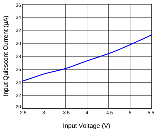
Input Quiescent Current vs. Input Voltage
