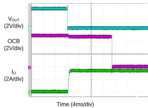
OCB Response during Over Load
