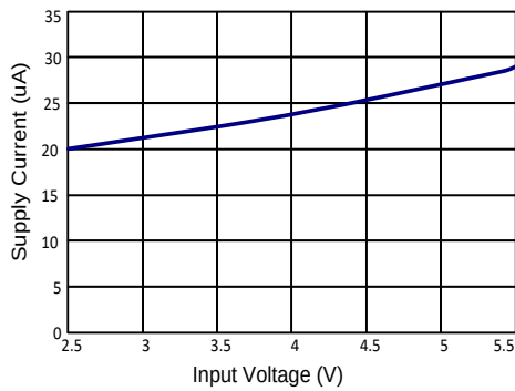
Supply Current vs. Input Voltage ( R_{LOAD}=10\Omega , C_{IN}=10\mu F , C_{OUT}=4.7\mu F )
