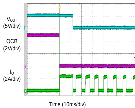
OCB Response during Short Circuit
