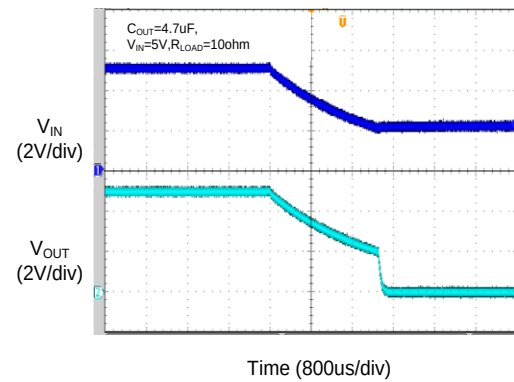
UVLO at Falling
