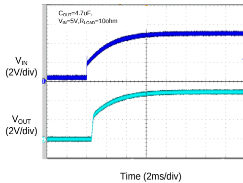
UVLO at Rising
