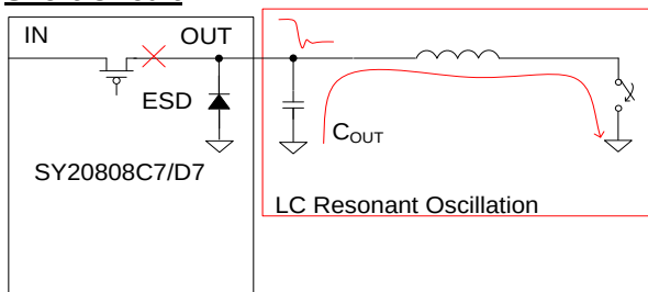
Figure 3. Equivalent Circuit
