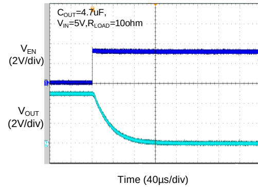
Turn OFF Response
