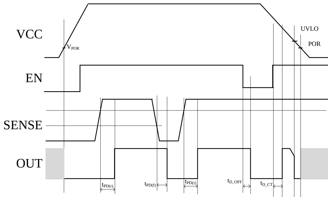
Figure3. SY28637F Sequence
