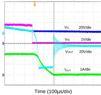
Loss of SYS GND with Inductive Load (V_S=28V, C_{VS}=C_{OUT}=Null, Z_{LOAD}=14\Omega+6mH, R_{DEN}=R_{IN}=10k\Omega, REF: GND\_SYS)
