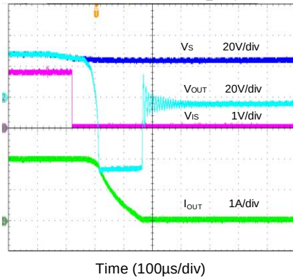
Loss of IC GND with Inductive Load (V_S=28V, C_{VS}=C_{OUT}=Null, Z_{LOAD}=14\Omega+6mH, R_{DEN}=R_{IN}=10k\Omega, REF: GND\_SYS)
