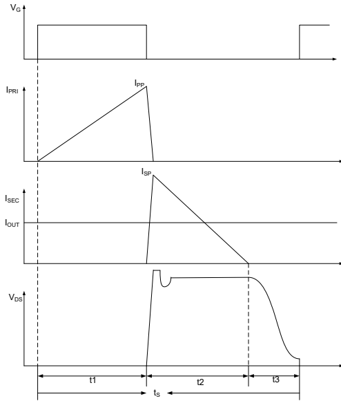
Fig.9 switching waveforms
