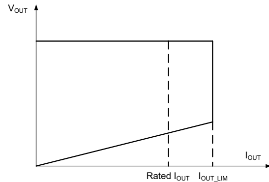
Fig.6 V-I curve
