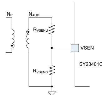
Fig. 6 Cable compensation
