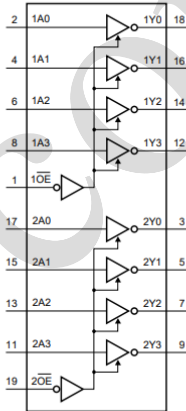
Figure 2. Functional diagram
