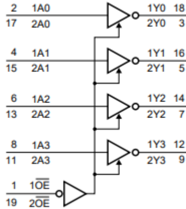
Figure 1. Logic symbol
