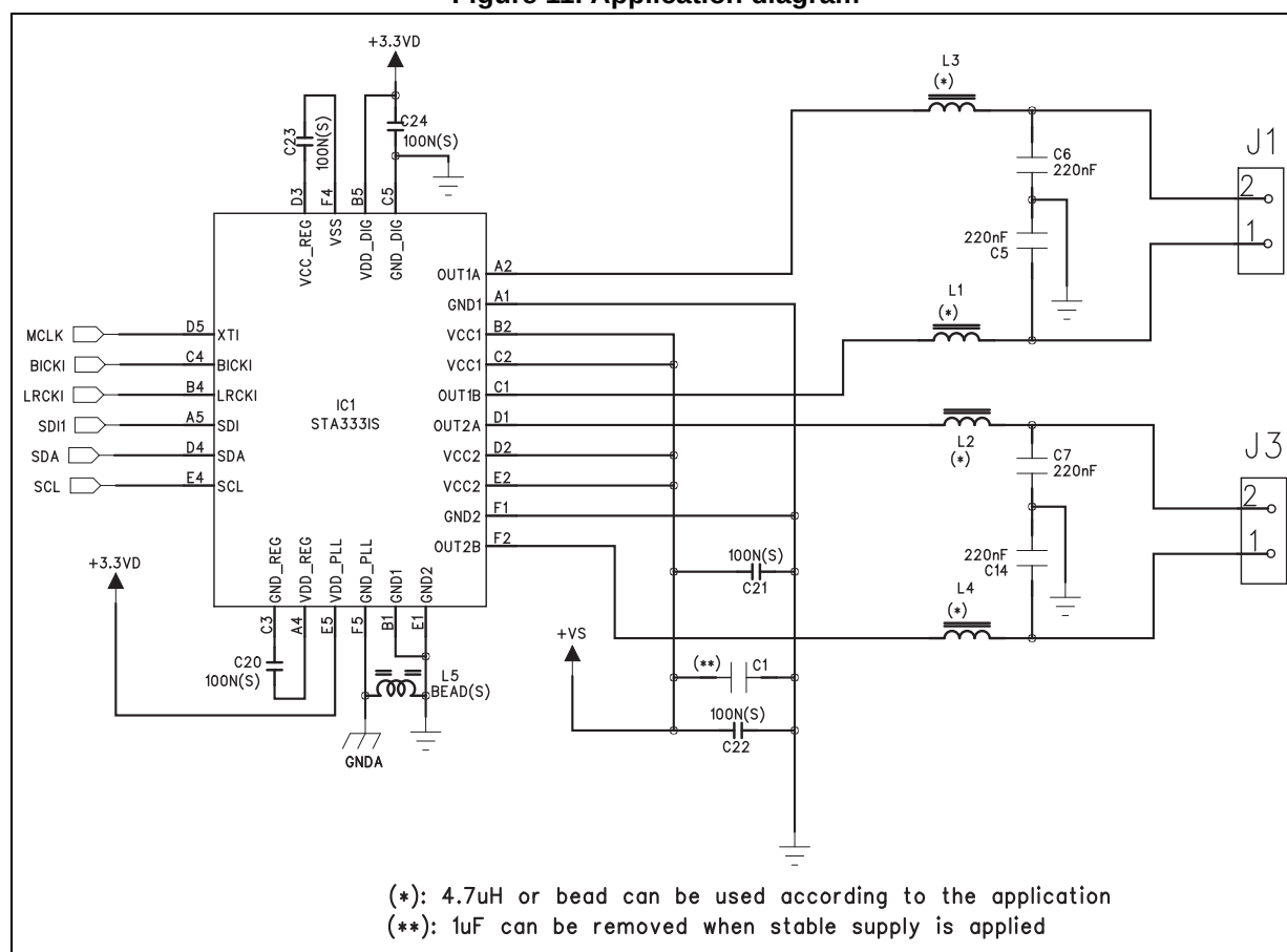
Figure 11. Application diagram
