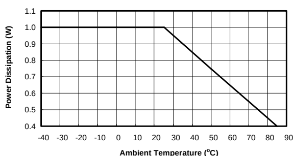
Figure 2. Derating Curves for APL3527S Package
