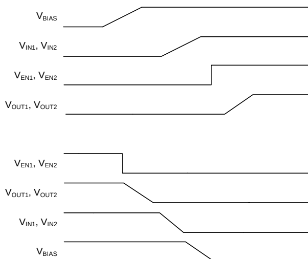
Figure 2. APL3533A Power Sequencing Diagram
