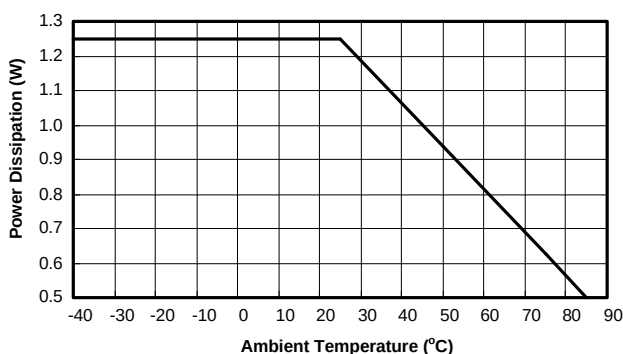
Figure 3. Derating Curves for APL3533A Package
