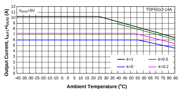
Figure 3. Derating Curves for APL3533A Package
