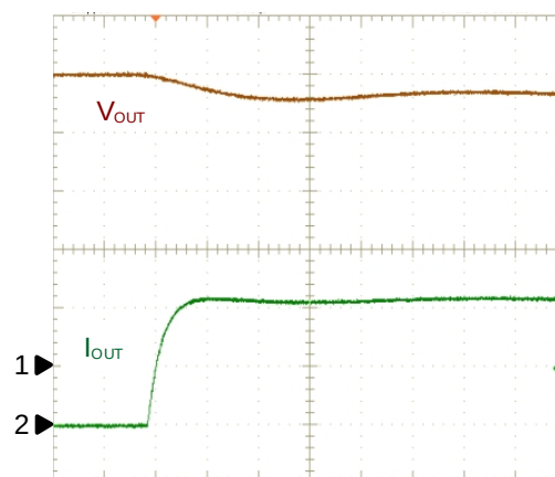
Load-Transient Response
