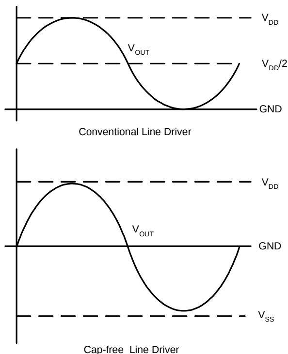
Figure 1. Cap-free Operation
