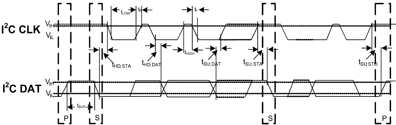
Timing Diagram
