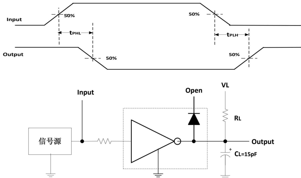
Fig. 6 Transmission delay waveform
