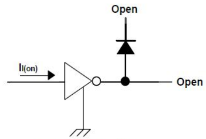
Fig.4 I_l Test Circuit
