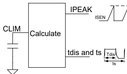
Figure 7. Current Sense
