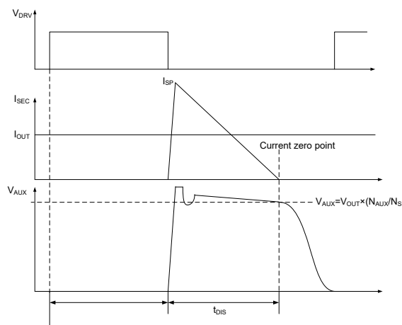
Figure 6. Auxiliary Winding Voltage Waveforms
