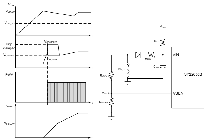
Figure 3. Startup
