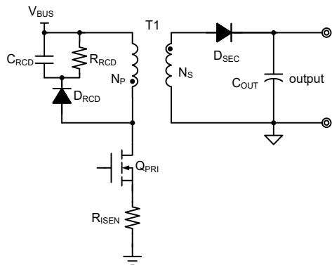
Figure 11. RCD Snubber
