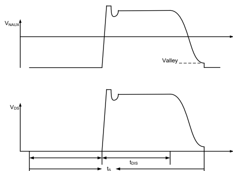
Figure 4. QR Operation
