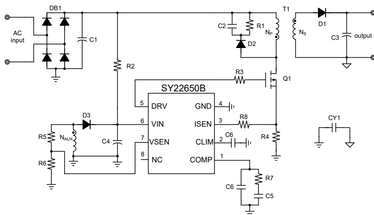
Figure 1. Schematic Diagram
