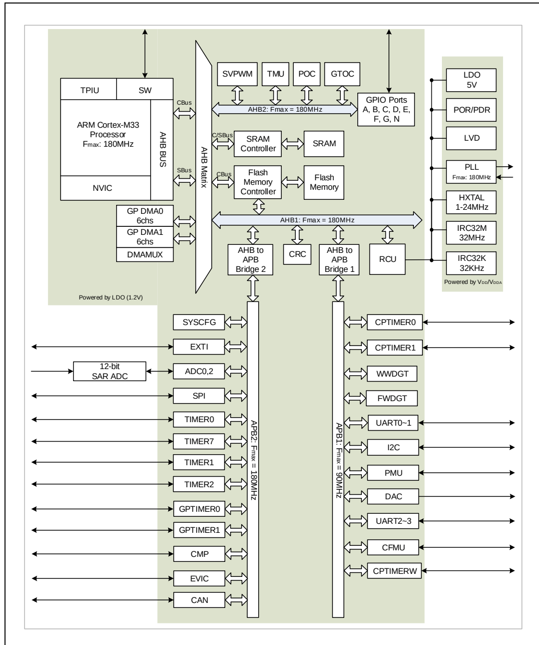
Figure 2-1. GD32M531xx block diagram
