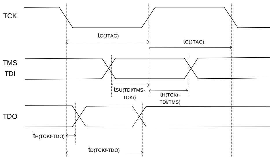
Figure 4-36. JTAG timing diagram
