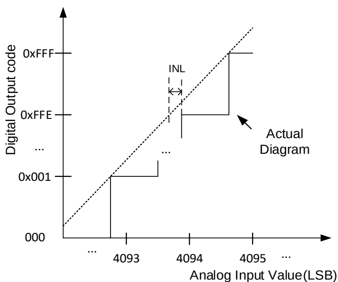
Figure 4-13. Integral linearity error
