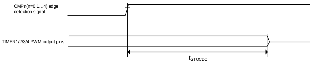
Figure 4-24. Output Disable Time for GTOC in Response to the Register Setting
