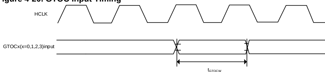
Figure 4-20. GTOC Input Timing
