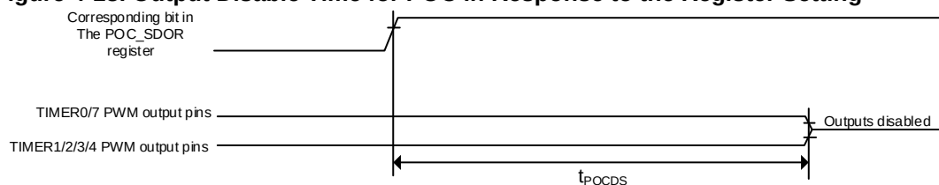
Figure 4-18. Output Disable Time for POC in Response to the Register Setting
