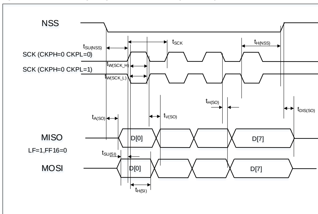
Figure 4-30. SPI timing diagram - slave mode(CKPH=0)
