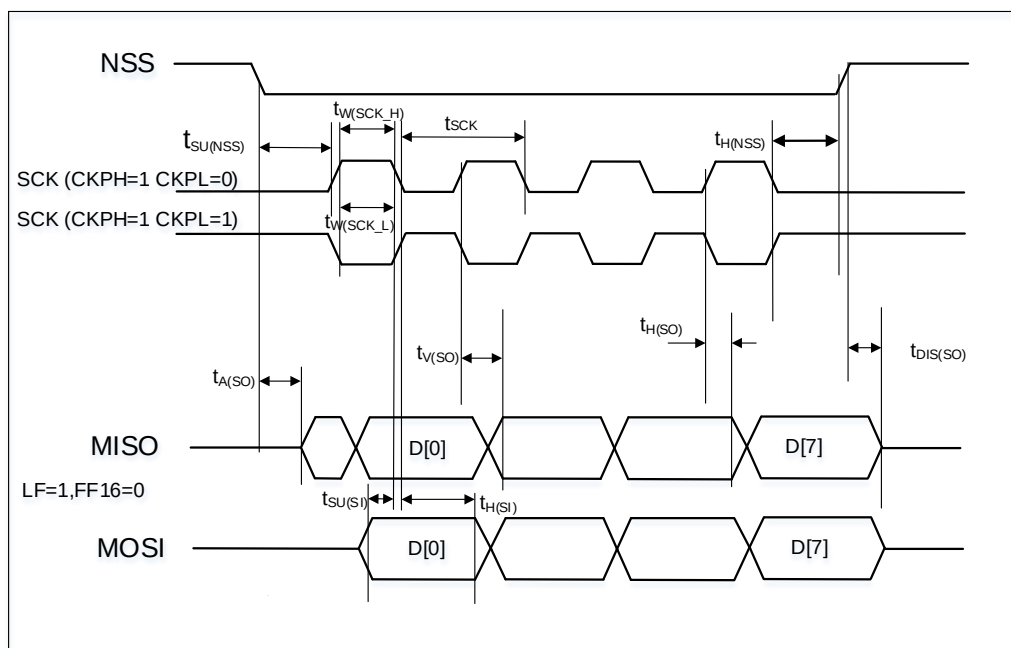
Figure 4-31. SPI timing diagram - slave mode(CKPH=1)
