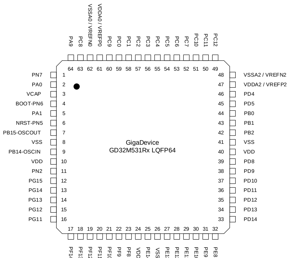
Figure 2-3. GD32M531Rx LQFP64 pinouts
