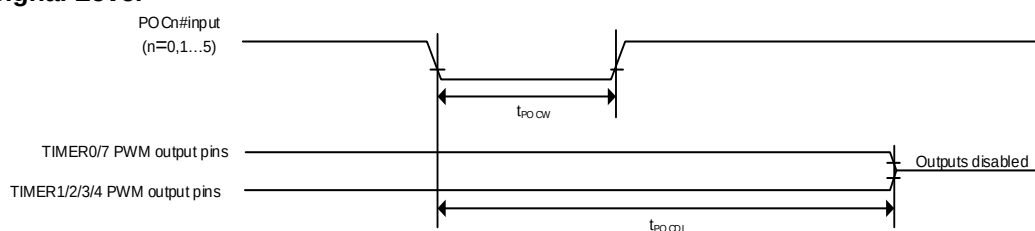
Figure 4-15. Output Disable Time for POC in Response to Transition of the POCn# Signal Level
