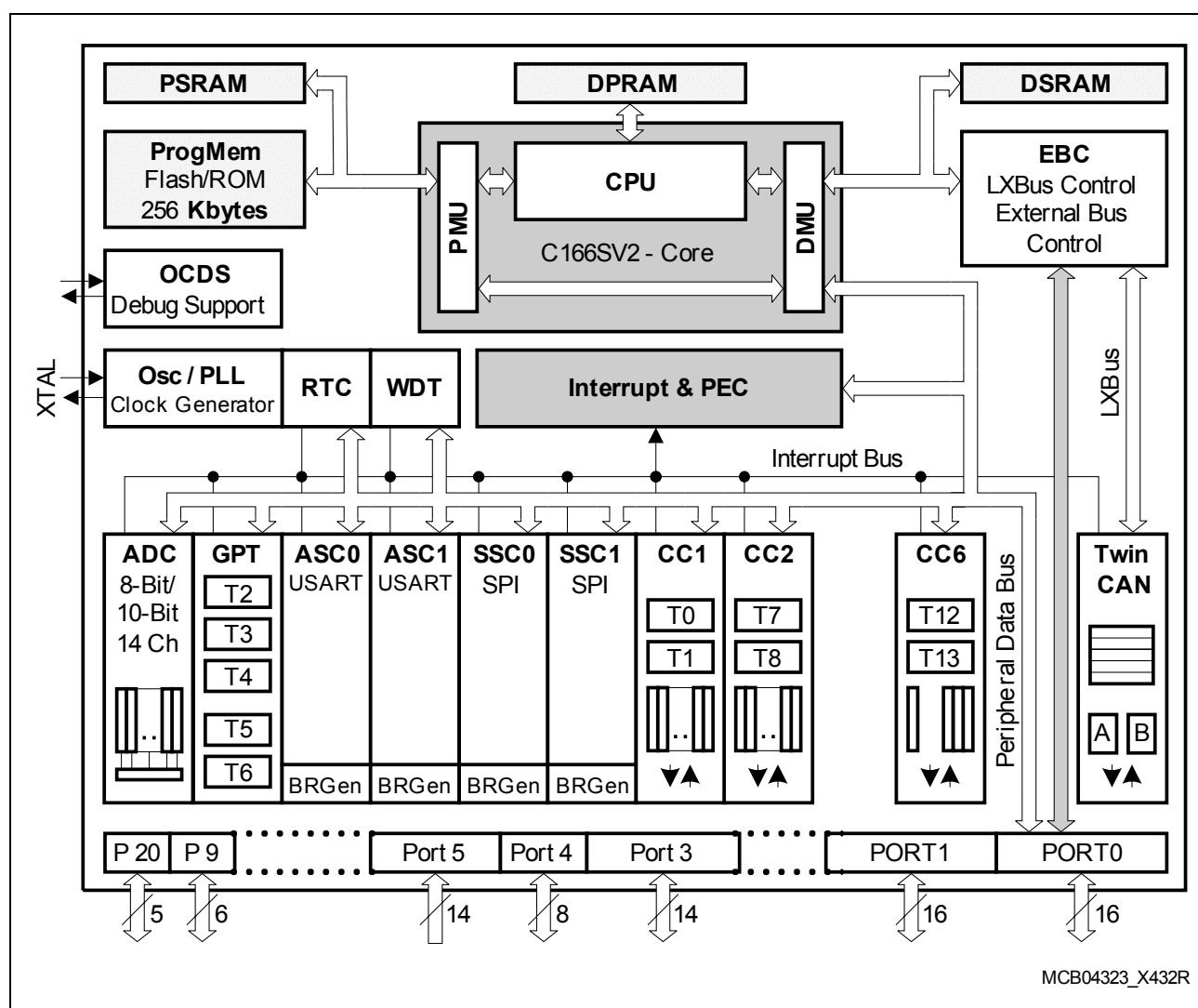
Figure 3 Block Diagram
