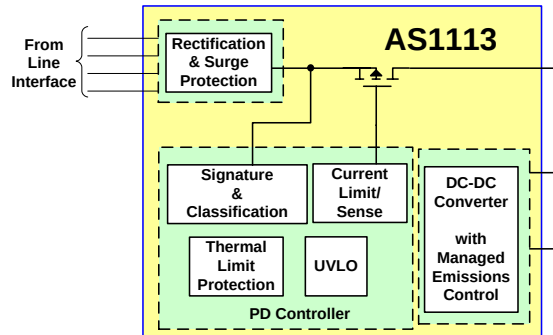
Figure 4. Top-Level Block Diagram of the AS1113
