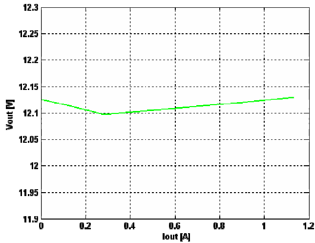
DCDC Load Regulation vs. I_{OUT} @ V_{IN}=48V , V_O=12V
