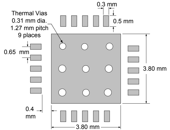
Figure 7. AS1113 PCB Footprint
