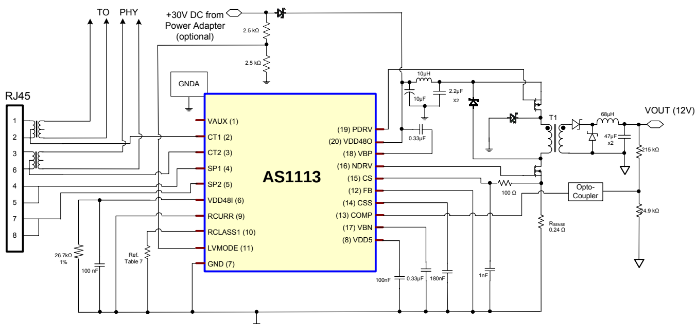
FIGURE 9. 10/100M WITH FORWARD DC-DC CONVERTER
