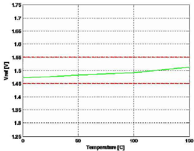
Error Amplifier Ref. Voltage vs. Junction Temperature
