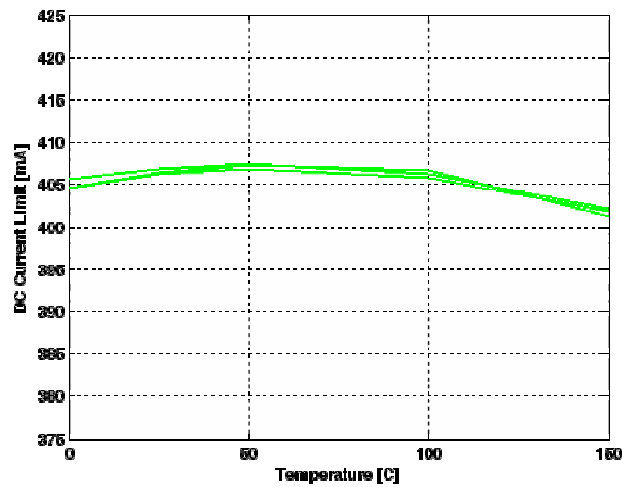
DC Current Limit vs. Junction Temperature
