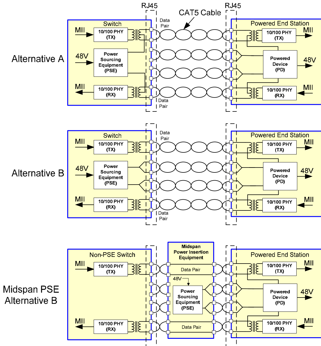
Figure 3. IEEE® Std. 802.3af-2003 Power Feeding Schemes for 10/100 Systems
