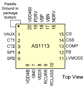
Figure 2. Pin-out Diagram
