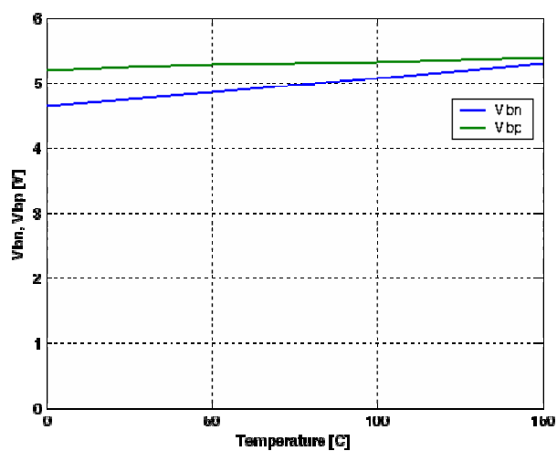
VBN &amp; VBP (VBP wrt VDD480) vs. Junction Temperature
