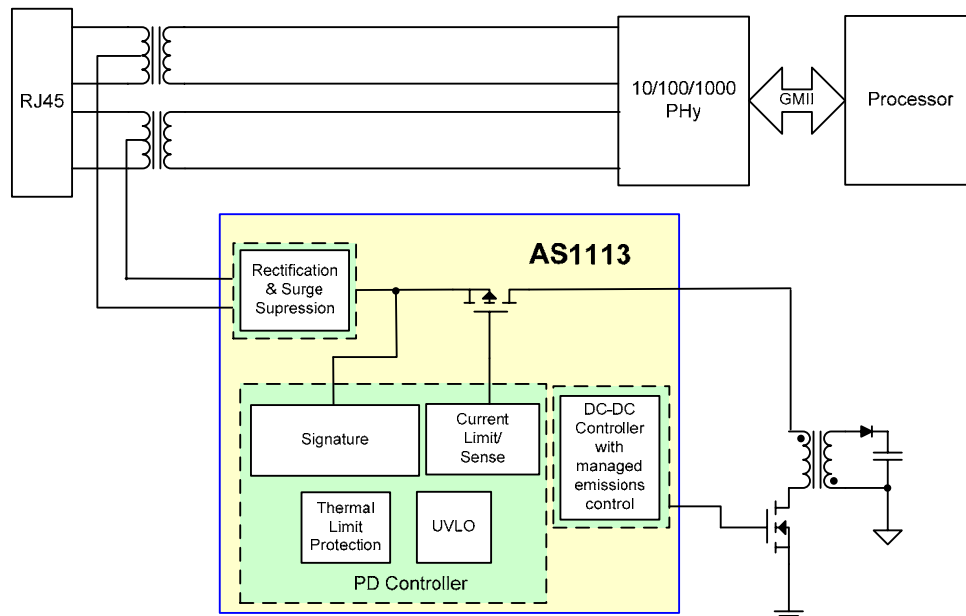
Figure 1. Typical Application Diagram for a Power over Ethernet PD (Flyback Converter)
