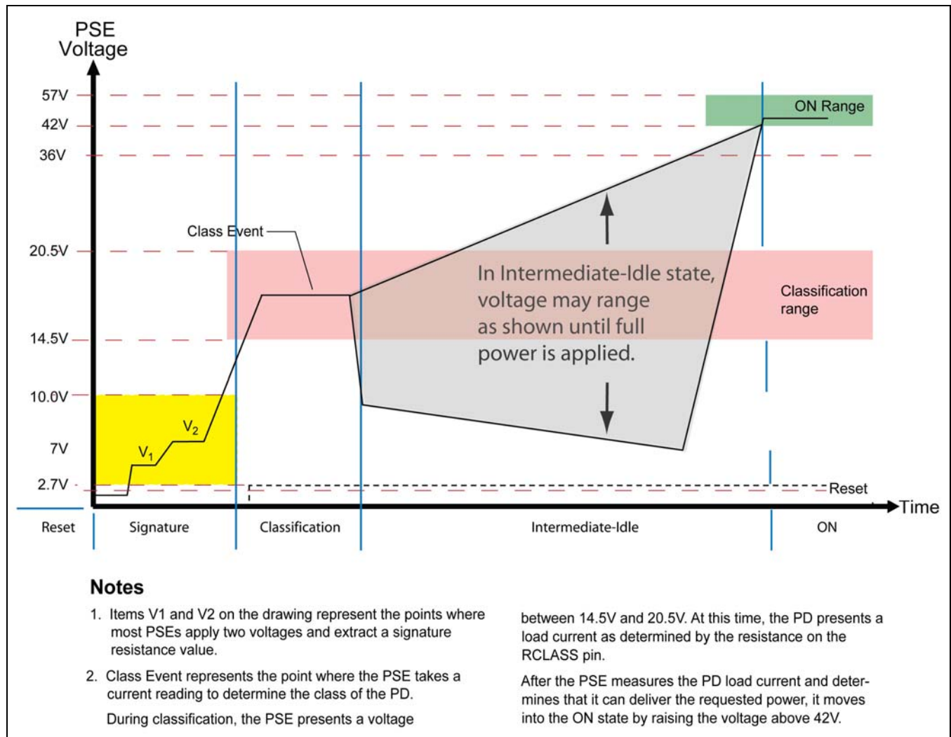
Figure 6. Representative Power-On waveform
