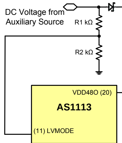
Figure 5. AS1113 LVMODE Connection
