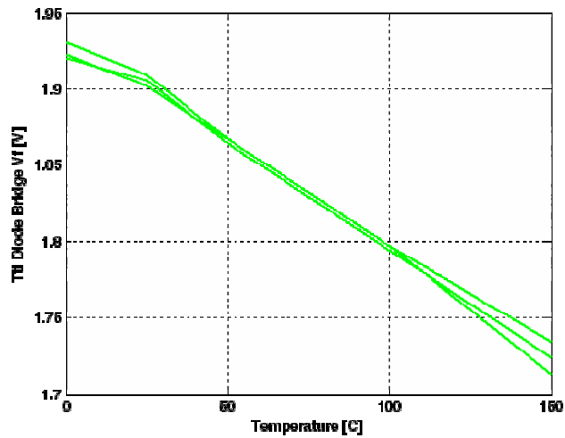
Full Load Diode Bridge V_F vs. Junction Temperature
