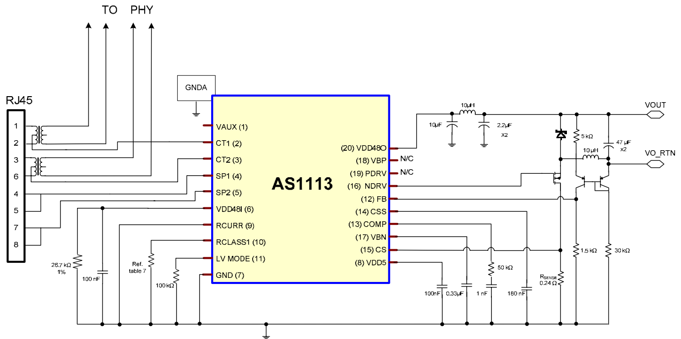
FIGURE 10. 10/100M WITH BUCK DC-DC CONVERTER
