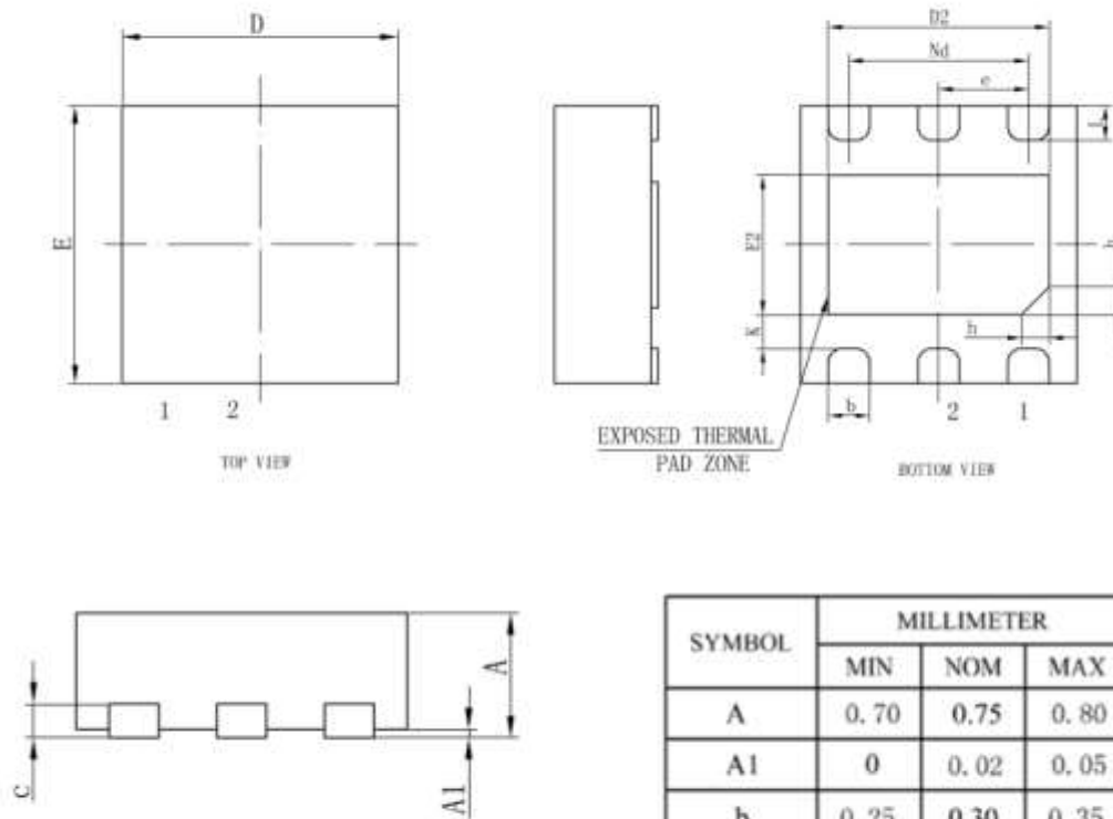
TDFN-6
