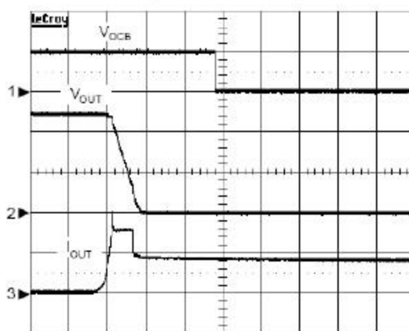
OCB Response with Ramped Load
