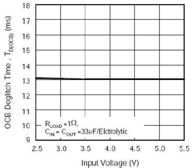
OCB Deglitch Time vs. Input Voltage
